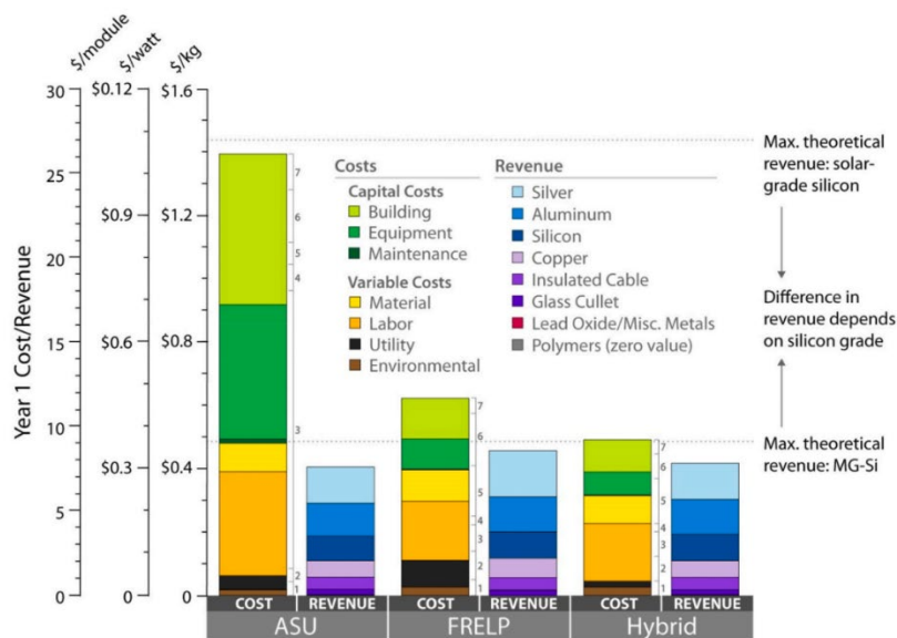
Figure 2: Technoeconomic assessment costs from three PV recycling processes (adapted from Cui et al., 2019). 8
